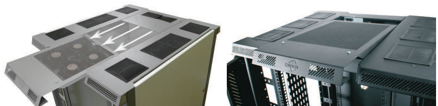
Images show QuickChange fan unit fitted (ServerSmart Cab/SmartCab versions only).
